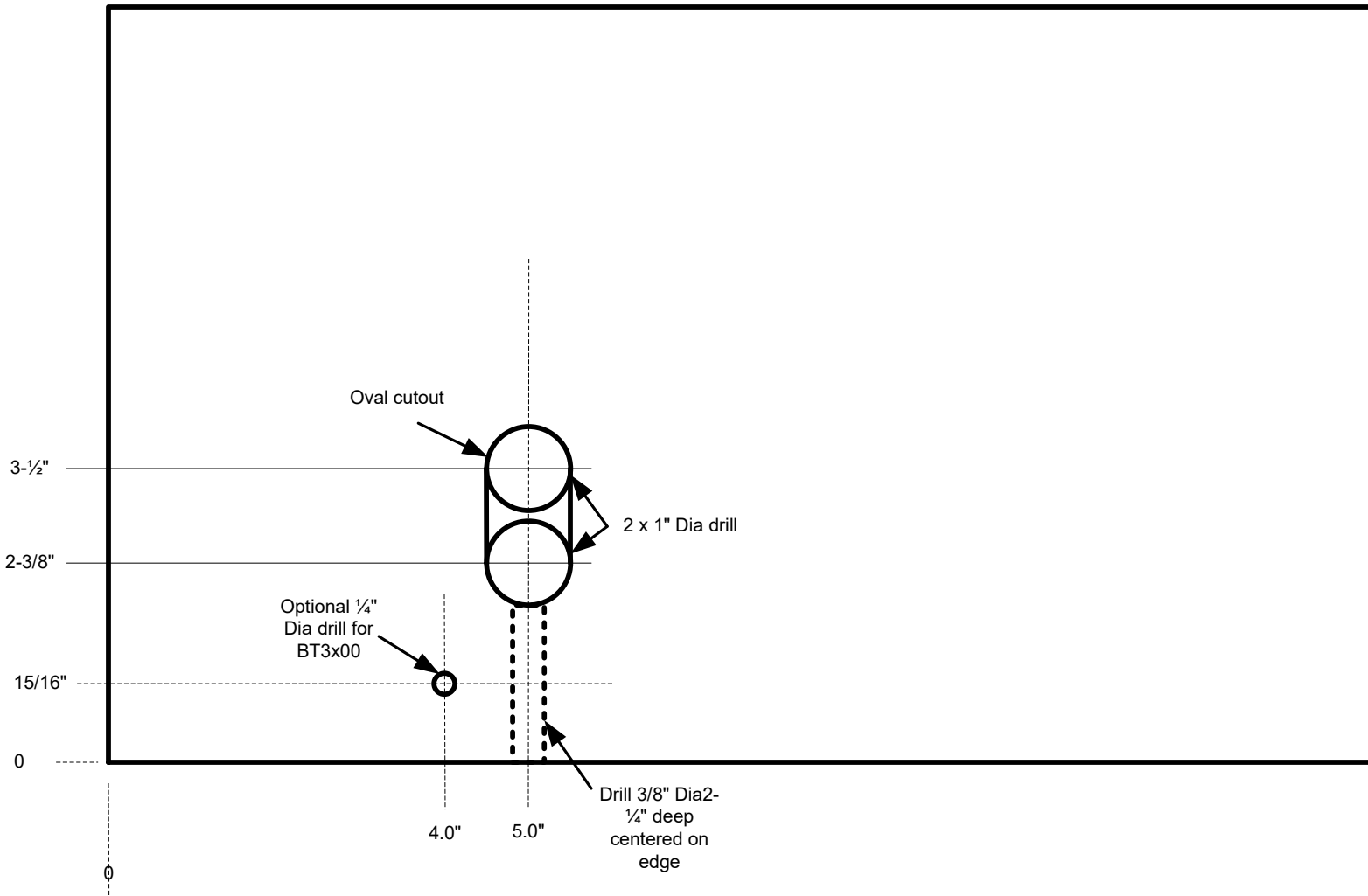
Tall Rip Fence for use with Rockler Fence Clamp and BT3x00 Material 3/4" Ply 24" long x 9" high Drawing shows one end, make other end identical mirror image.
